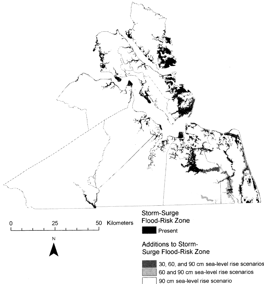
Figure 8. Storm surge flood-risk zone with post sea-level rise increases, Category 1 hurricanes at high tide.
